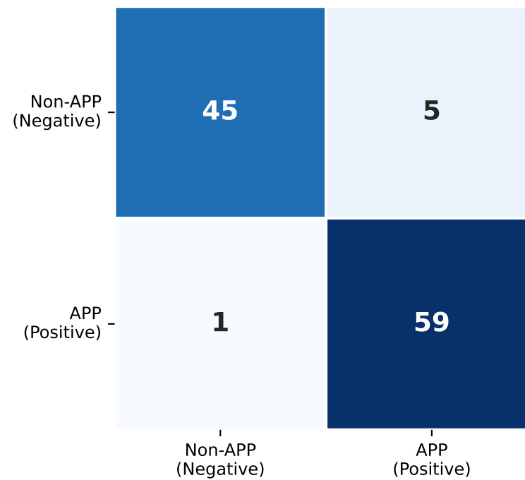
Model 5
