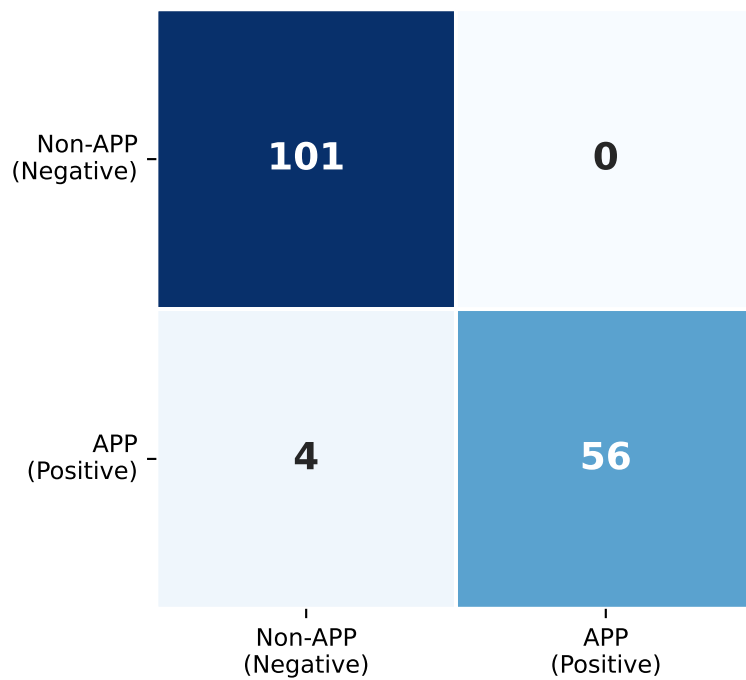
Model 4
