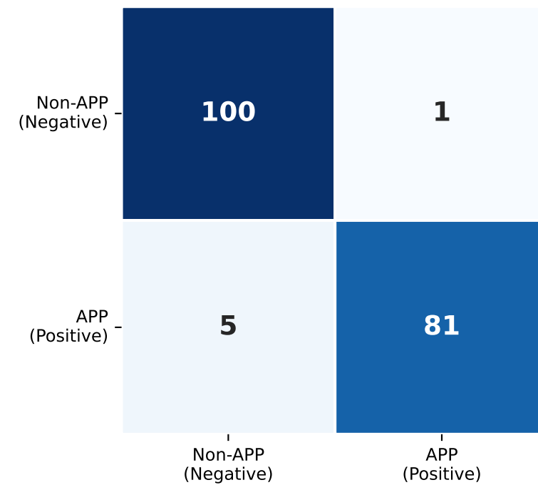
Model 6
